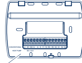
Performance PRO Wallplate & Terminal Connections
