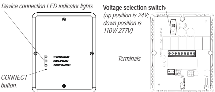
Figure 2: RW205 Receiver: LED indicators and CONNECT button.
