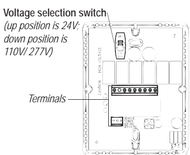
Figure 3: RW205 Receiver with front cover removed.
