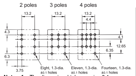
PCB Processing Dimensions (Bottom View)
