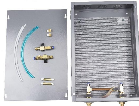
BVA-5-PW2 Un-Assembled
