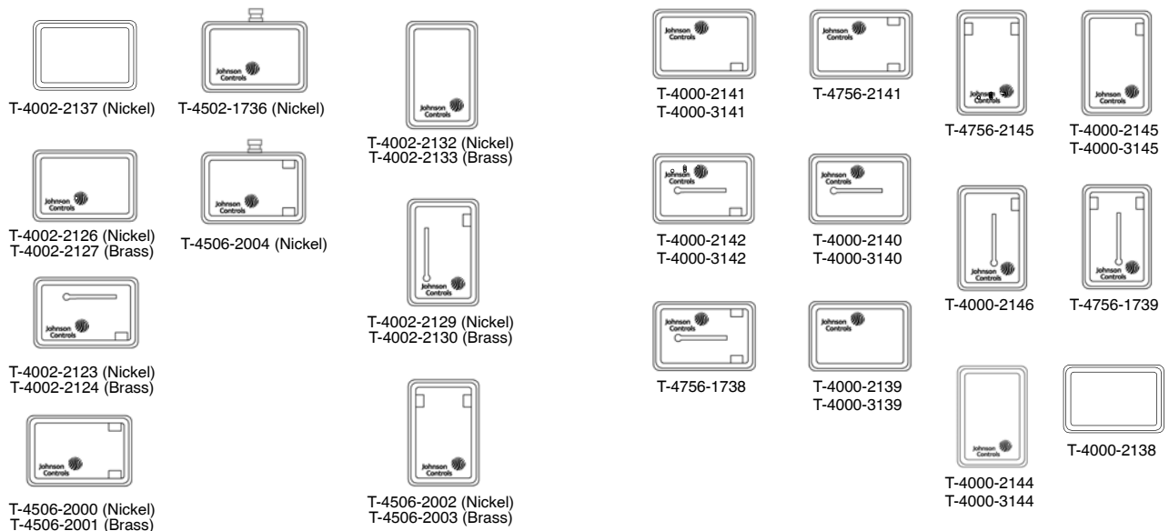
T-4000 Series Covers with Faceplates
