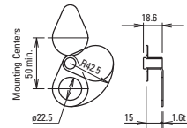
OLW-C Metal Button Guard
