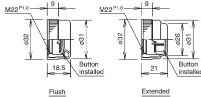
AW-RP1B Round Plastic Bezel
