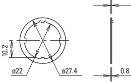
OGL-31 Anti-Rotation Ring
