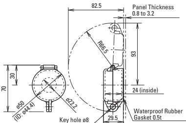
HW9Z-KL1 Lock-out Adaptor
