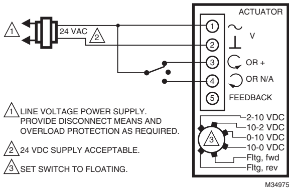
Fig. 16. MS7505 with Floating Control (Floating mode setting).
