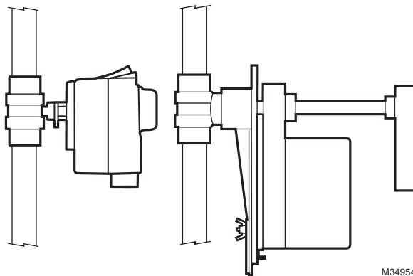
Fig. 4. Vertical valve installation.
