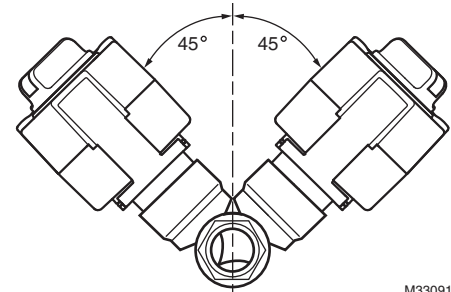
Fig. 5. Acceptable valve angle from vertical.
