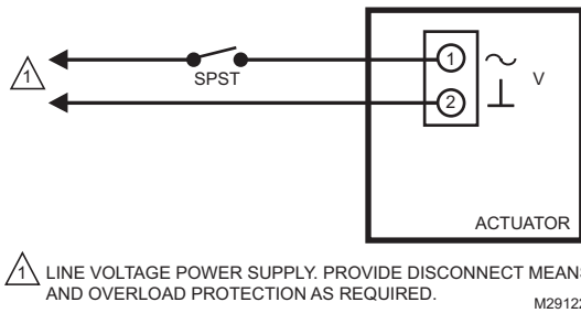
Fig. 20. MS4105 line voltage (120V) two-position control.
