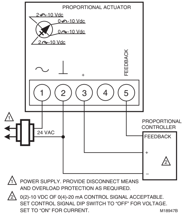
Fig. 8. MN7505 with Modulating Control.
