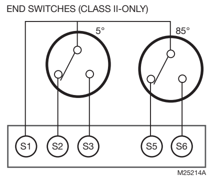
Fig. 9. Wiring for model with aux./end switches.
