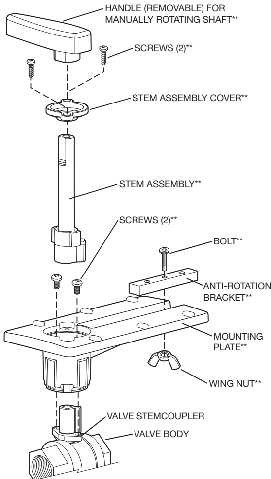
Fig. 3. Valve assembly exploded view.
