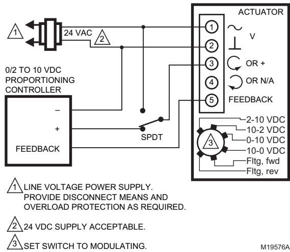
Fig. 17. MS7505 with override to full open (Modulating mode setting).
