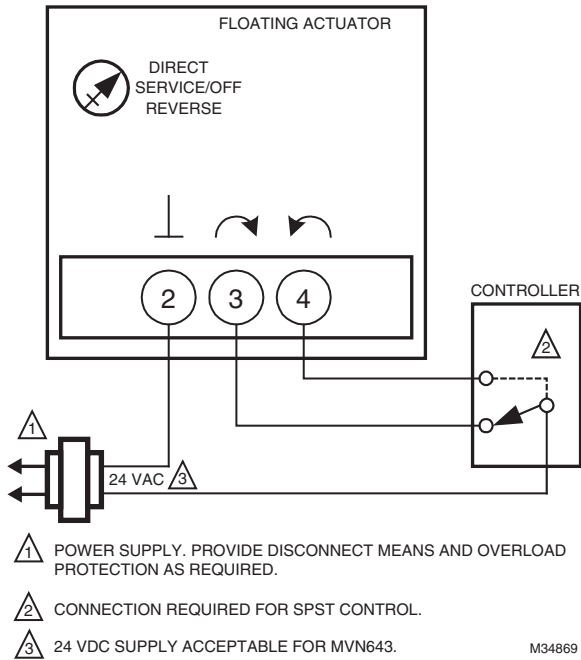
Fig. 6. MN6105 with On/Off Control.
