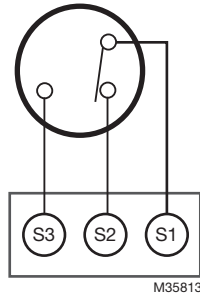
Fig. 21. Wiring for model with aux./end switches.
