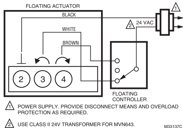
Fig. 10. MVN613 or MVN643 with Floating Control.
