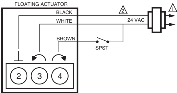
Fig. 11. MVN613 or MVN643 with 2-Position Control.
