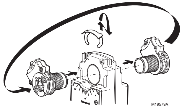
Fig. 23. Mounting shaft coupling to actuator opposite side.
