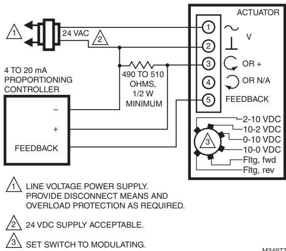
Fig. 19. MS7505 with Proportioning Controllers (Modulating mode setting).
