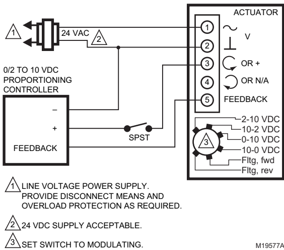
Fig. 18. MS7505 with override to full closed (Modulating mode setting).
