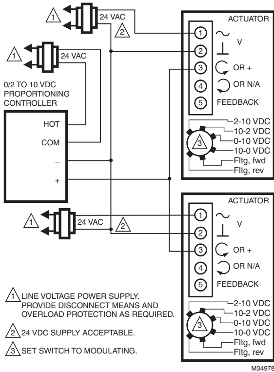
Fig. 22. MS7505 with Proportioning controllers operating multiple actuators (Modulating mode setting).
