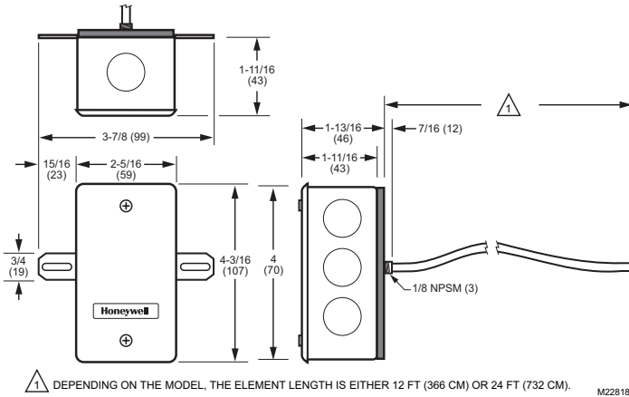
Fig. 4. C7021R, C7023R, C7041R dimensions in in. (mm).
