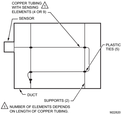
Fig. 5. Duct cross section showing method of installing C7021R, C7023R, C7041R Averaging Electronic Sensor.
