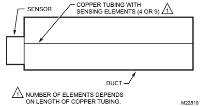
Fig. 6. Duct cross section showing method of installing C7021R, C7023R, C7041R in a multizone system.
