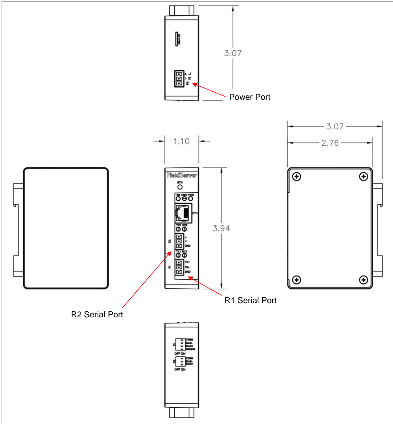
Figure 25: BACnet Router Dimensions
