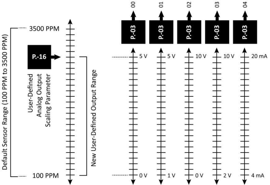
Figure 15. Analog Output Scaling Options
