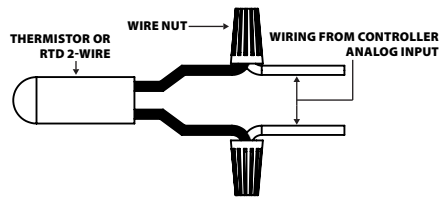
FIGURE 3: TEMPERATURE WIRING
