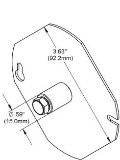
Fig. 6: Ceiling Mount Cover (ZPS-ACC05)
