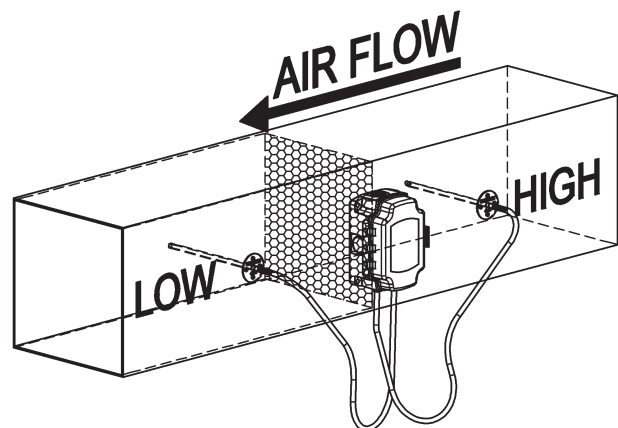
Fig. 3: Measuring air filter pressure drop with BAPI ZPS Pressure Transmitter mounted on a duct and two BAPI ZPS-ACC07 in duct.
