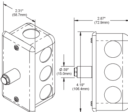
Fig. 7: Ceiling Mount Cover & J-Box (ZPS-ACC06)
