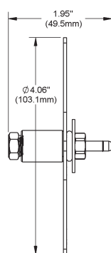
Fig. 6: Ceiling Mount Cover (ZPS-ACC05)
