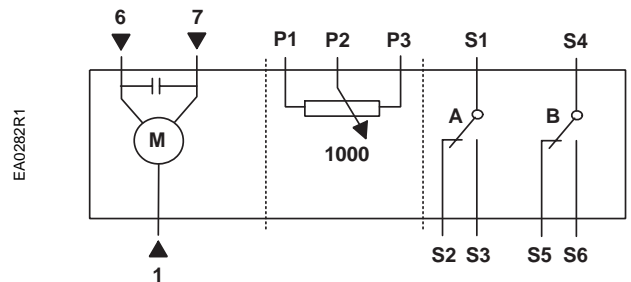
Figure 18. GBB/GIB13x Three-position Control, 24 Vac.
