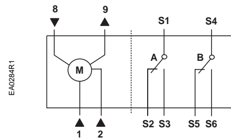
Figure 17. GBB/GIB16x Modulating Control, 24 Vac.
