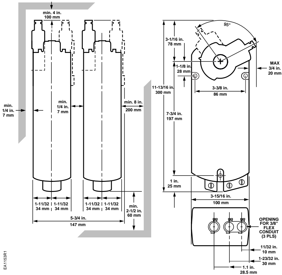
Figure 22. Dimensions and Service Envelope of the GIB Actuators in Tandem Application in Inches (mm).
