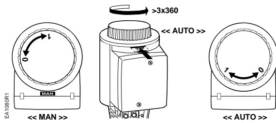
Figure 14. Manual Override in Manual and Automatic Position.
