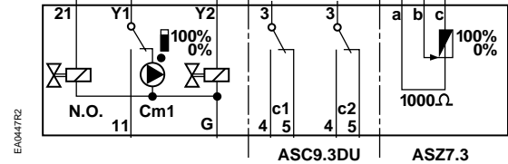
Figure 13. Spring Return SKD82.51U.
