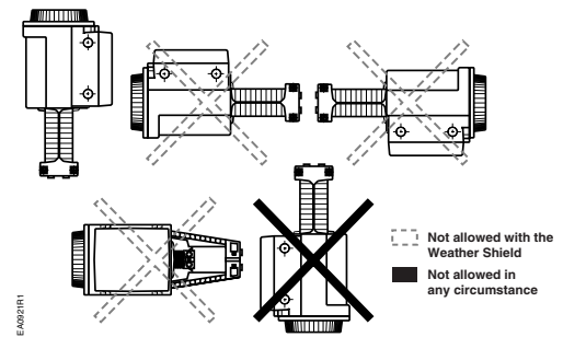
Figure 1. Acceptable Mounting Positions.
