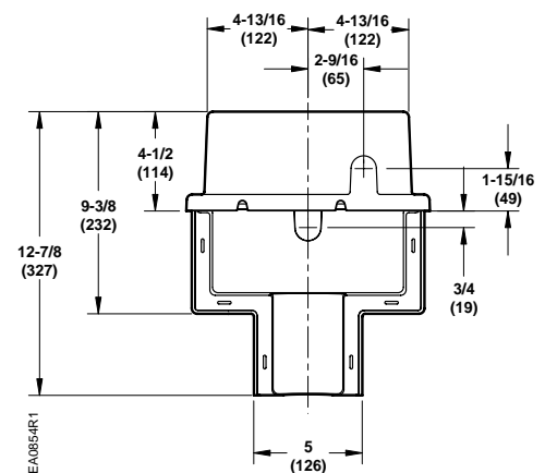
Figure 16. Dimensions of the 599-10071 Weather Shield in inches (mm).
