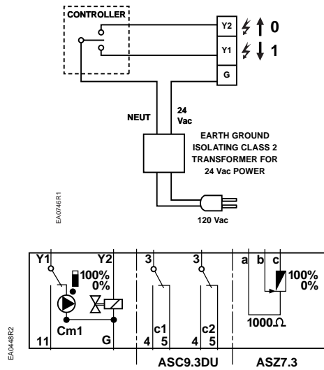
Figure 12. Non-Spring Return SKD82.50U.
