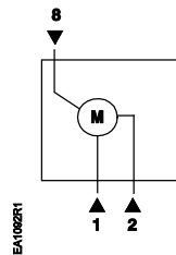
Figure 28. GDE161.1N 0 to 10 Vdc Modulating Control Wiring Diagram.
