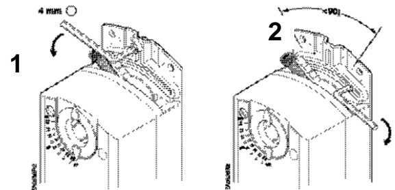
Figure 23. Moving the Mechanical Range Stop.
