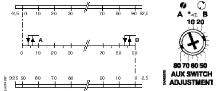
Figure 17. Adjustable Switching Values for the Dual Auxiliary Switches.
