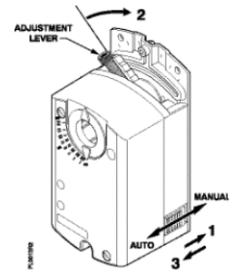
Figure 22. Manual Override.
