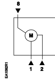
Figure 25. GDE161.1T Wiring Diagram.
