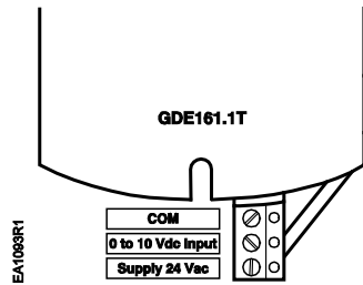
Figure 24. GDE161.1T Terminal Strip.
