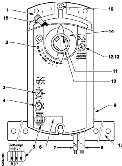
Figure 11. Parts of the Actuator.
