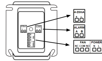
Figure 2 Line Voltage Detector (12 Series) Rear View and Connectors
