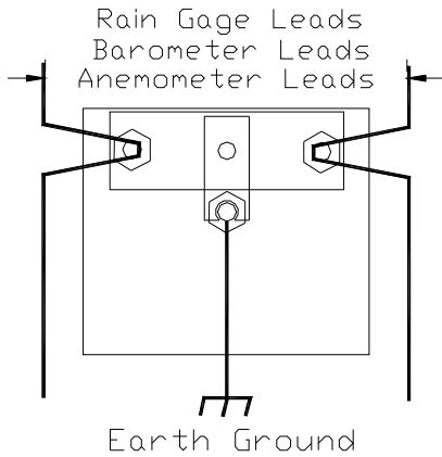
Model A96-100
